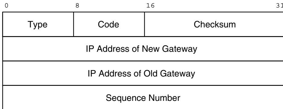
Figure 3 ICMP mobile host movement notification and reply message format
