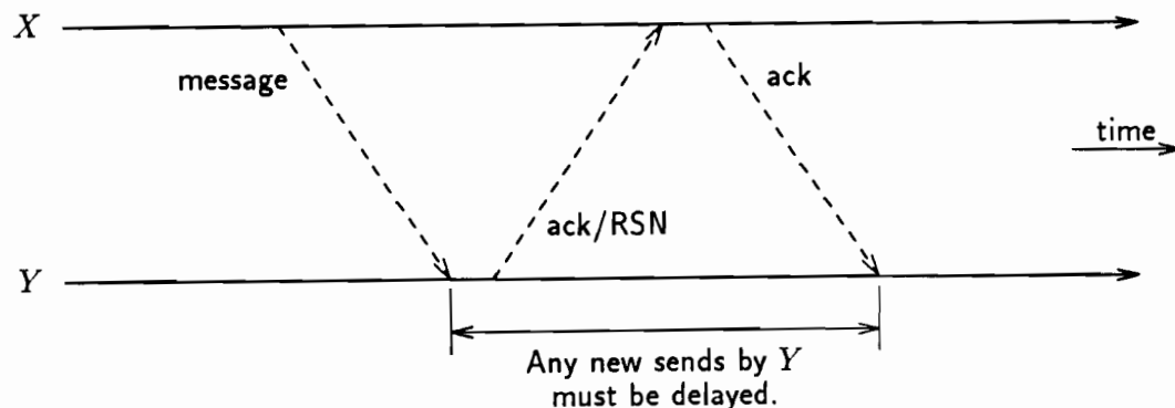
FIGURE 3: Operation of the message logging protocol in the absence of transmission errors
