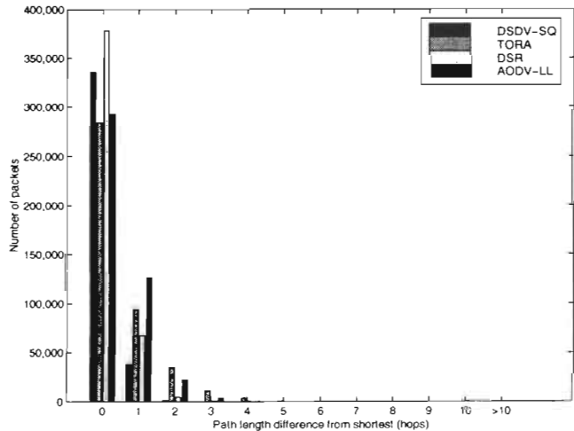
Figure 6 Difference between the number of hops each packet took to reach its destination and the optimal number of hops required. Data is for 20 sources.
