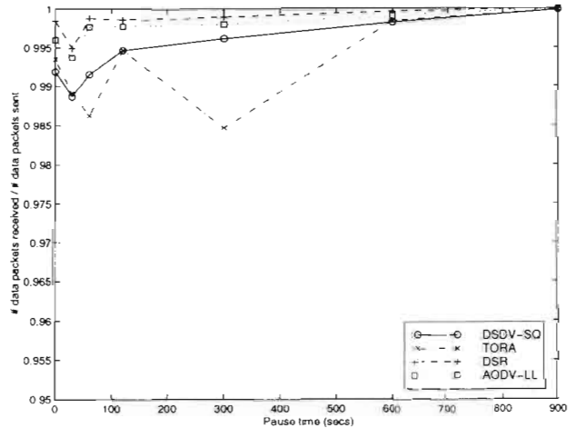
Figure 7 Comparison of the fraction of application data packets successfully delivered as a function of pause time. Speed is 1 m/s.
