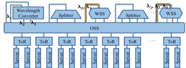
Figure 1: Programmable optical network architecture with optical components and subsystems to generate multicast groups.
