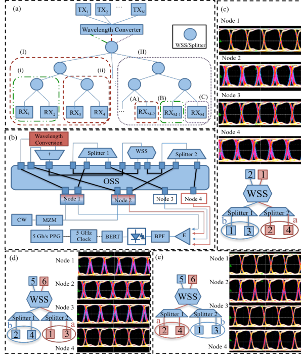
Figure 2: Demonstration of agile and efficient reconfiguration in multicasting groups in a tree architecture with N transmitters and M receivers, (b) Experimental setup of programmable optical network architecture supporting multiple multicast groups and fast switching, (c), Multicast data delivery on the same tree, (d) and (e) Fine time scale multicasting group assignment.
