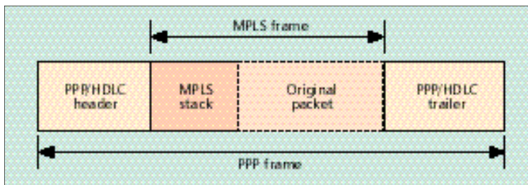
■ Figure 6. MPLS encoding for PPP over SONET/SDH links.
