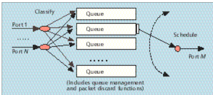
■ Figure 1. Per-hop classification, queuing, and scheduling.
