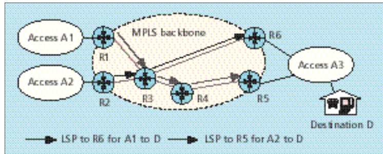
■ Figure 9. Explicitly routed LSPs as tunnels.
