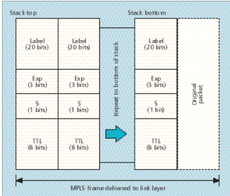
Figure 5. MPLS label stack encoding for packet-oriented transport.
