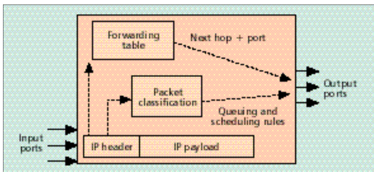
■ Figure 3. A simplified NIF node forwarding engine.
