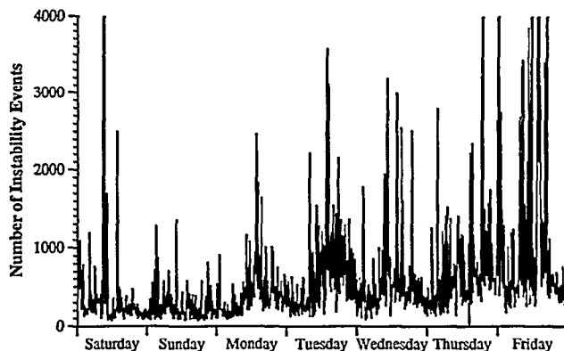
Figure 4: Representative week of raw forwarding instability updates (August 3 through 9, 1996) aggregated at ten minute intervals.
