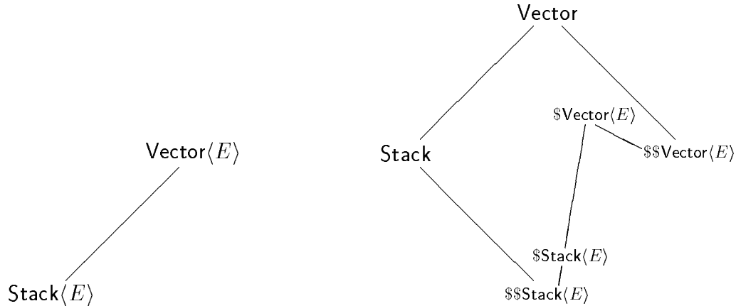
Figure 1: A Simple Parametric Type Hierarchy and its JVM Class Representation
