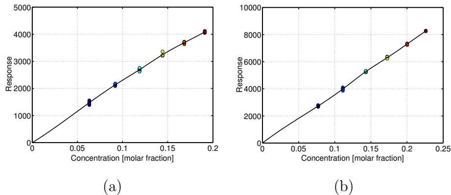
Fig. 3. Two examples of eNose sensor responses, illustrating their linearity: a) a metal-oxide sensor response vs. amyl formate concentration; b) a quartz-microbalance sensor response vs. toluene concentration. The dots are the measurements, and the solid line is an interpolation by piecewise cubic spline interpolation. Molar fractions are measured in poly ethylen glycol 400 solution.
