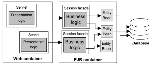
Figure 3. Session façade design pattern.
