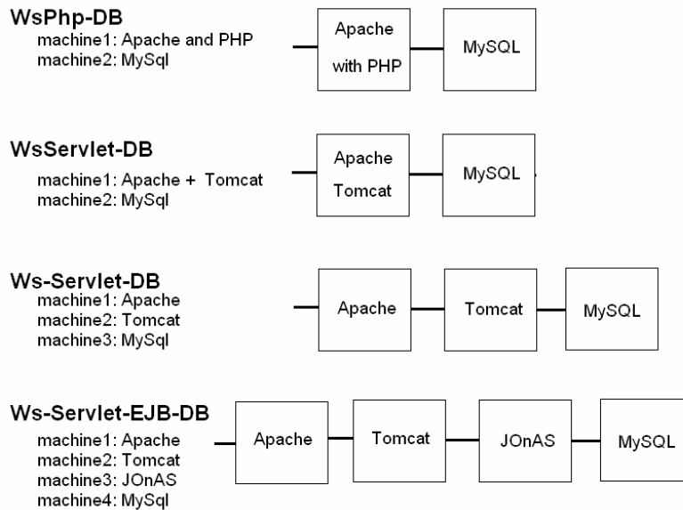
Figure 4. The four software and hardware configurations evaluated.
