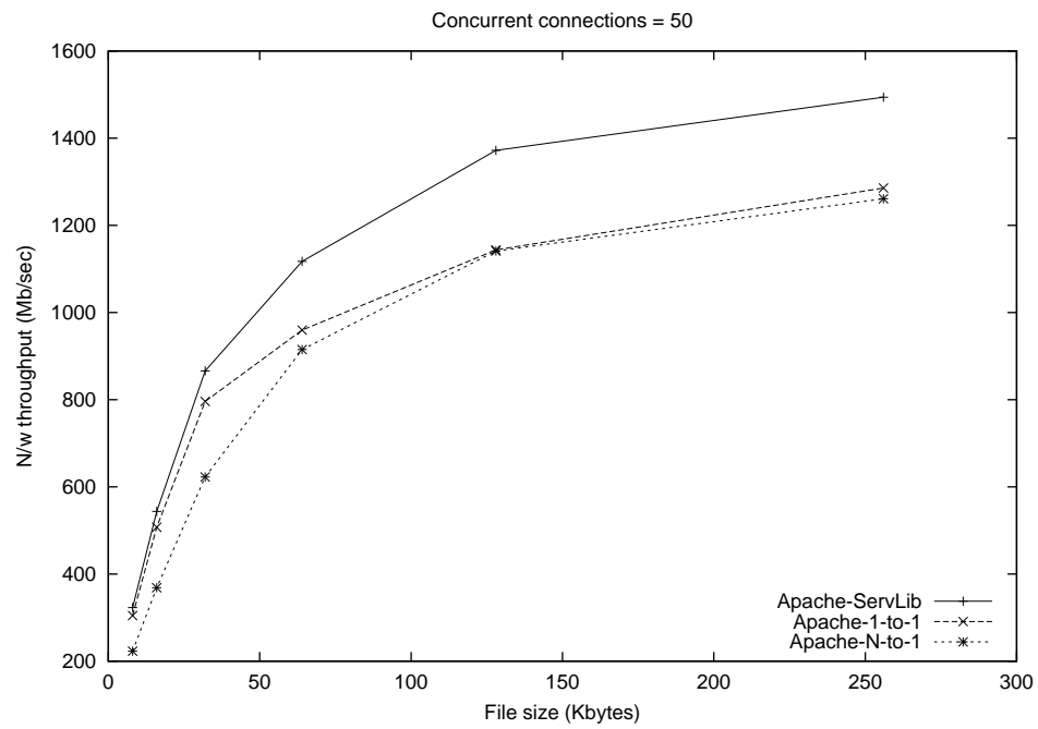
Figure 4.3 : Network throughput with varying file sizes, 50 concurrent connections
