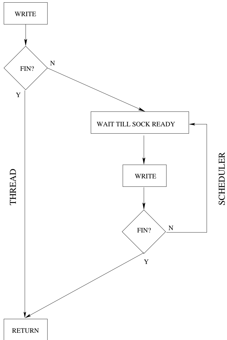
Figure 3.2 : Handling large writes in ServLib
