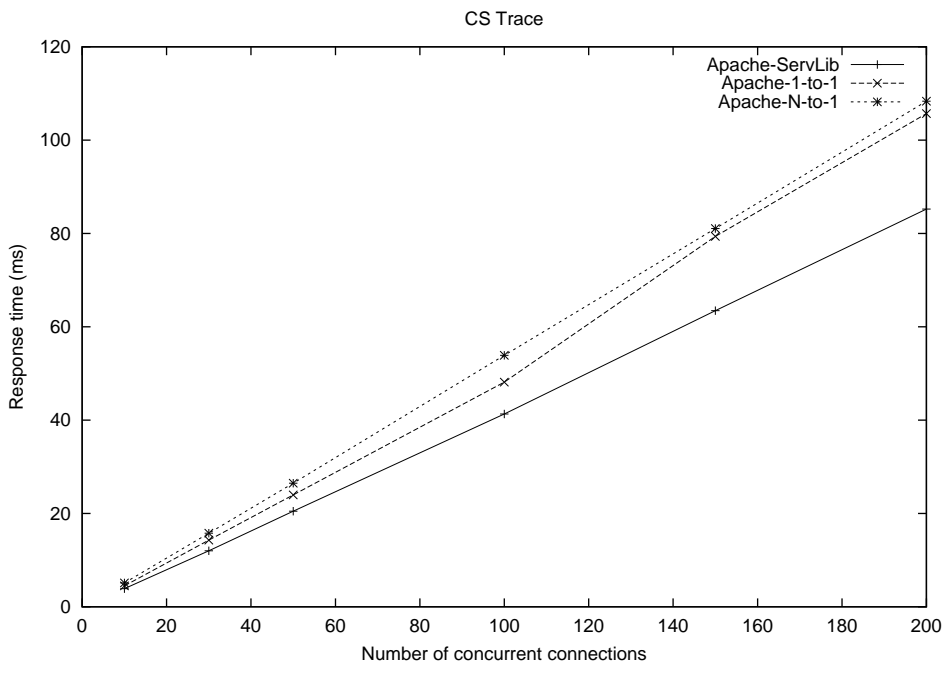
Figure 4.10 : Response time for CS trace with varying number of concurrent connections
