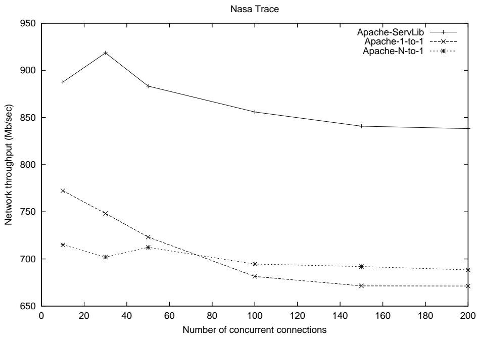
Figure 4.11 : Network throughput for Nasa trace with varying number of concurrent connections
