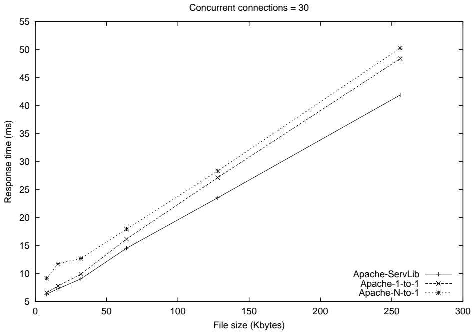
Figure 4.5 : Response time with varying file sizes, 30 concurrent connections
