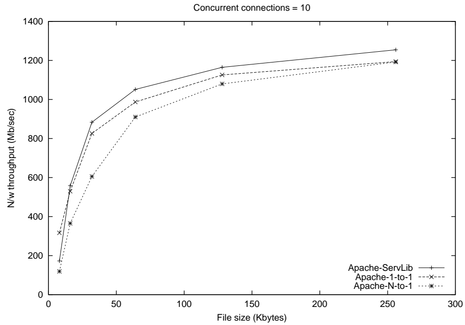
Figure 4.1 : Network throughput with varying file sizes, 10 concurrent connections
