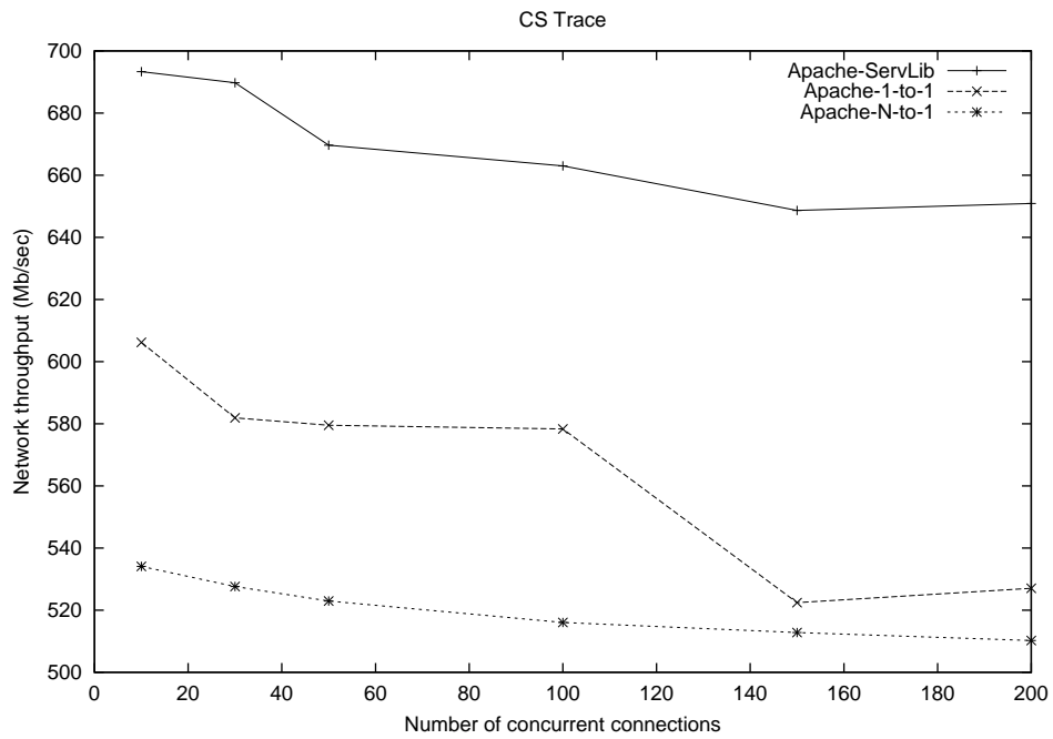
Figure 4.9 : Network throughput for CS trace with varying number of concurrent connections
