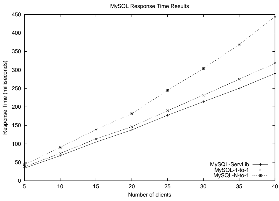
Figure 4.14 : MySQL response times with varying number of clients
