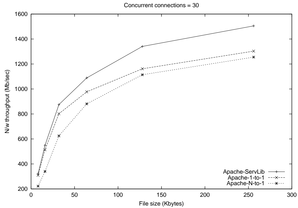
Figure 4.2 : Network throughput with varying file sizes, 30 concurrent connections
