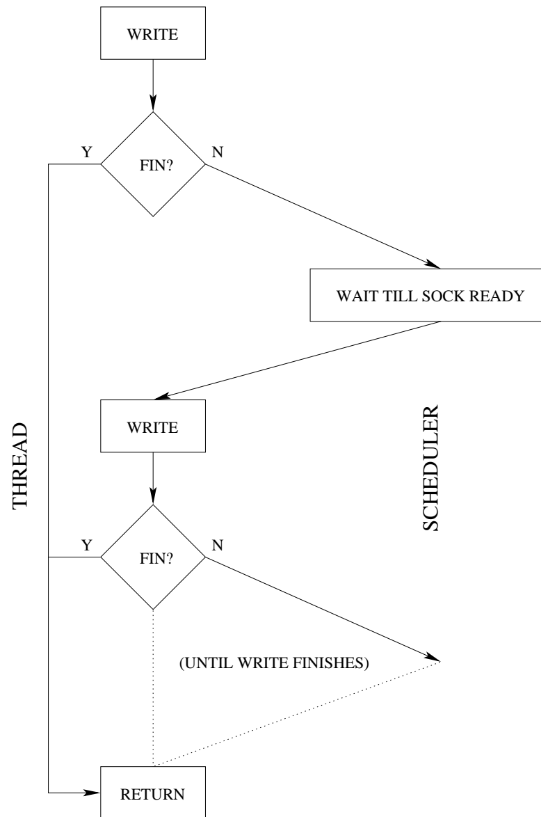
Figure 3.1 : Handling large writes in N-to-1 thread libraries
