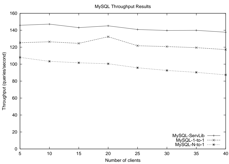
Figure 4.13 : MySQL throughput with varying number of clients
