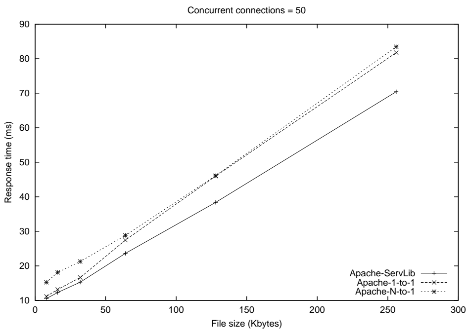
Figure 4.6 : Response time with varying file sizes, 50 concurrent connections
