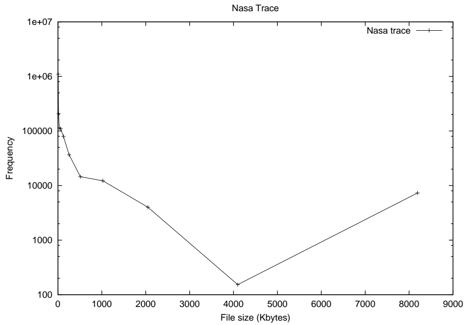
Figure 4.8 : Request distribution for NASA trace with increasing file size
