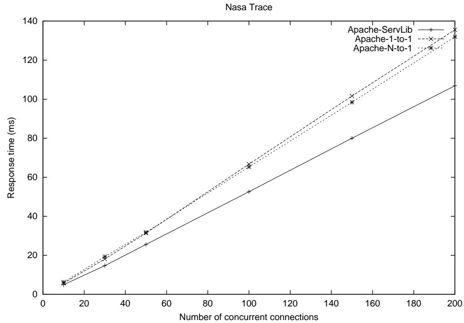
Figure 4.12 : Response time for Nasa trace with varying number of concurrent connections
