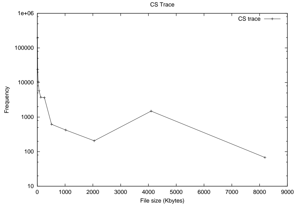
Figure 4.7 : Request distribution for CS trace with increasing file size
