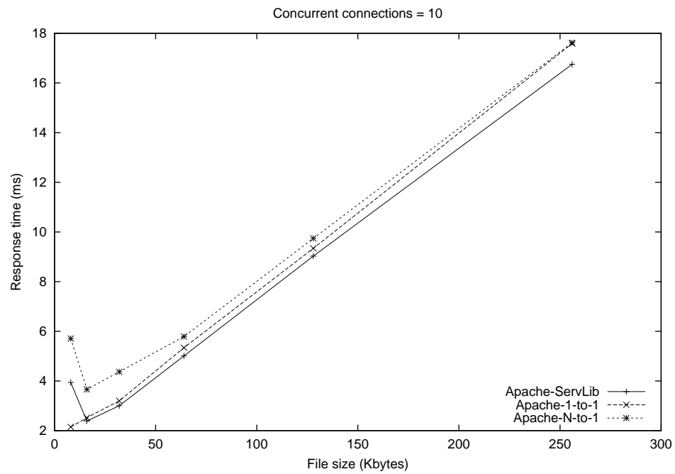
Figure 4.4 : Response time with varying file sizes, 10 concurrent connections
