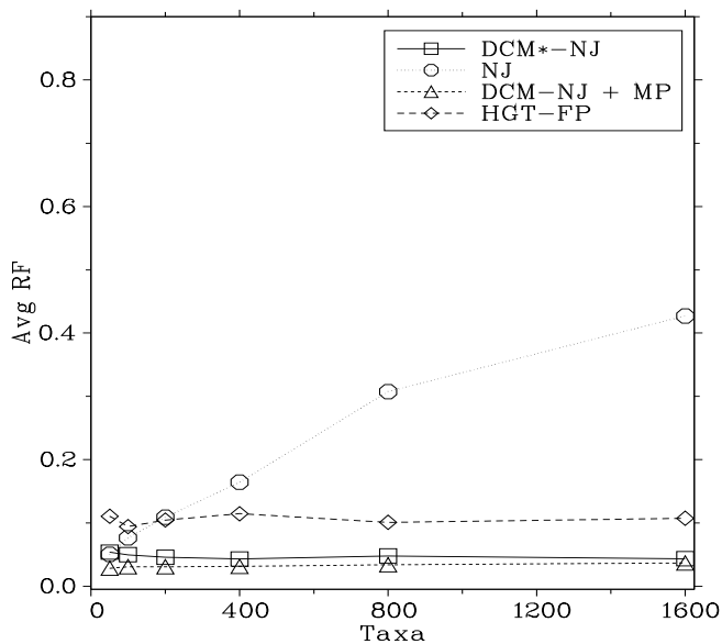
Fig. 9. DCM-NJ+MP vs. DCM*-NJ vs. NJ vs. HGT+FP on random trees under the K2P+Gamma model. Sequence length is 1000. Average branch length is 0.05.
