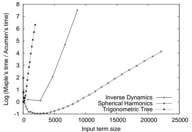
(b) Acumen is exponentially faster than Maple.
