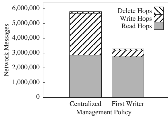
Figure 4. Comparison of locality as measured by network traffic for the Centralized and First Writer management policies.
