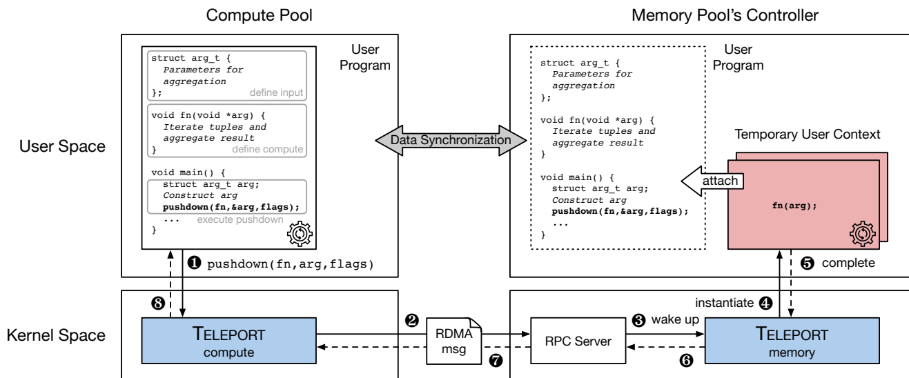
Figure 5: TELEPORT architecture.
