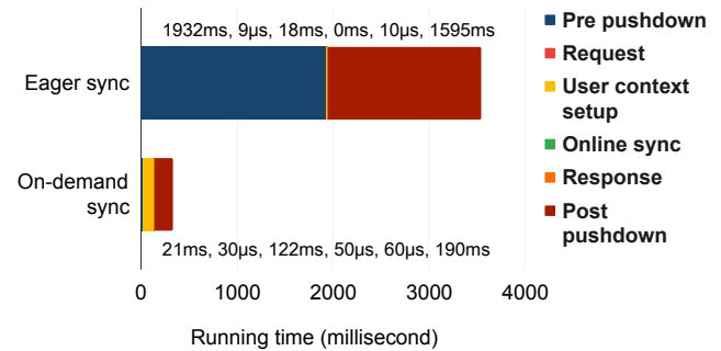
Figure 20: The breakdown of TELEPORT performance in different data sync methods with 1 GB compute-local cache.
