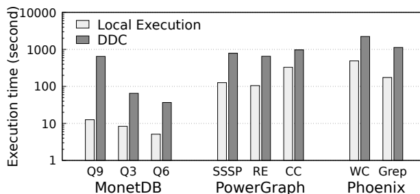
Figure 3: DDC performance overhead compared to a monolithic server. For DBMS (MonetDB), we show three TPC-H queries that have the highest disaggregation cost; for graph processing (PowerGraph) and MapReduce (Phoenix), we show popular benchmark queries (details are in Section 7).
