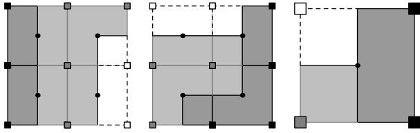
Figure 11: Three multi-material quadtrees and their dual contours.
