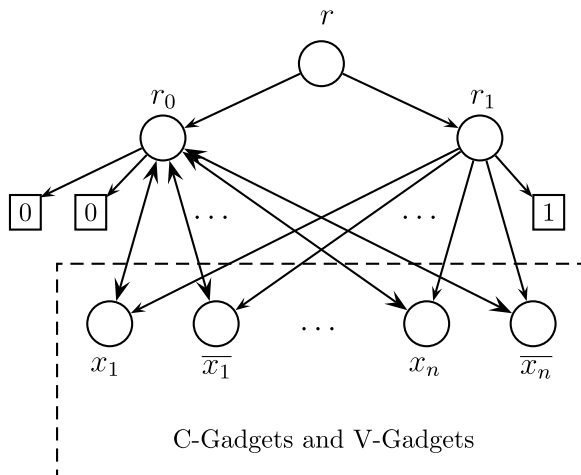
Fig. 3 The partition gadget and the whole network
