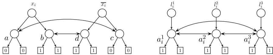
Fig. 2 The V-Gadget (left) and the C-Gadget (right)
