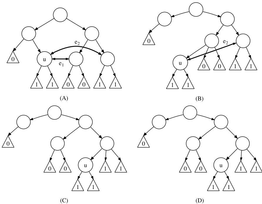
Fig. 4 An illustration for Fact 5.5
