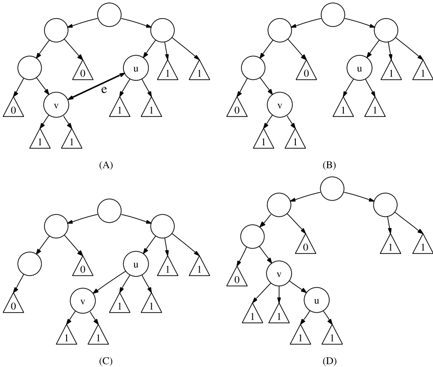
Fig. 1 An example of a phylogenetic network whose leaves are labeled by a single character, and the trees resulting from the possible assignments to the b-edge e in the network
