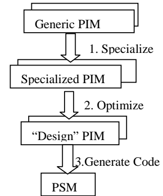
Figure 1: Steps in transforming a PIM to a PSM
