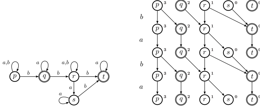
■ Figure 1 Left, the NBW \mathcal{A} , in which all states are initial. Right, the rejecting run DAG G of \mathcal{A} on w = babaabaaabaaaa \dots . Nodes are superscripted with the prospective ranks of Section 2.
