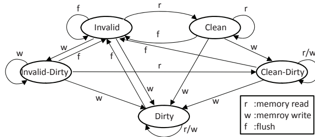
Fig. 2: State transition diagram for the cache protocol of ModelLF .
